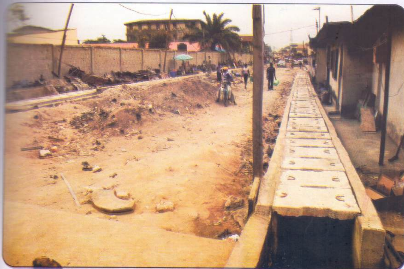
After Construction of 1800m drainage system with double wall reinforced concrete and a concrete covered slab
