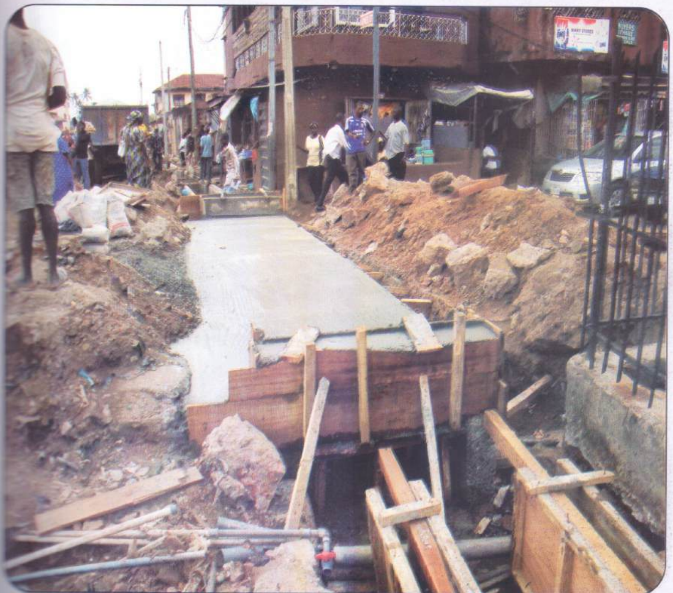
Completed Reinforced Concrete Culvert along Apapa Road to prevent Flood
