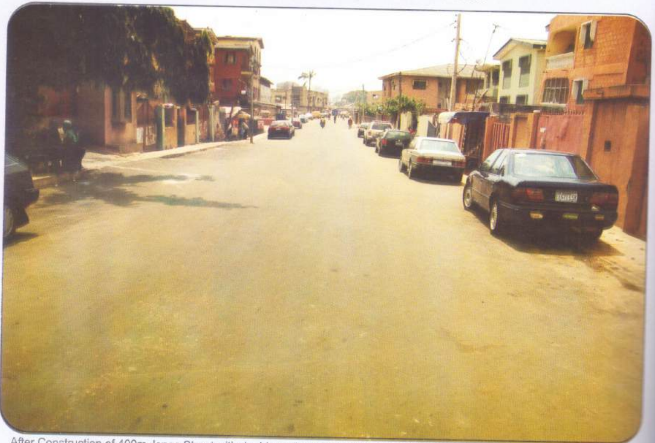
After Construction of 400m Jones Street with double wall reinforced concrete drainage system and a concrete covered slab
